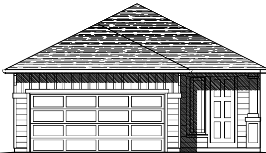
FRONT ELEVATION "E"
